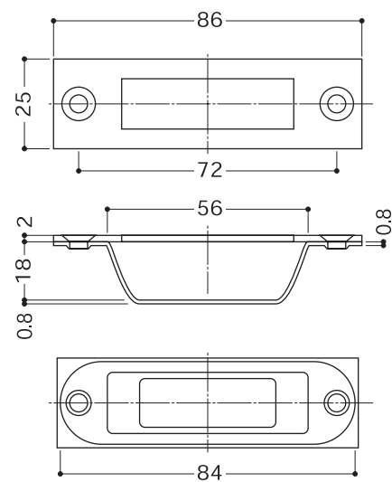
面付用受
