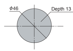
Cut out for 431 door pull
