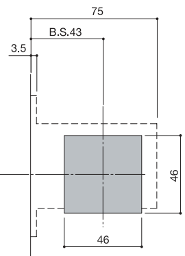
432 Cut out for lock case
