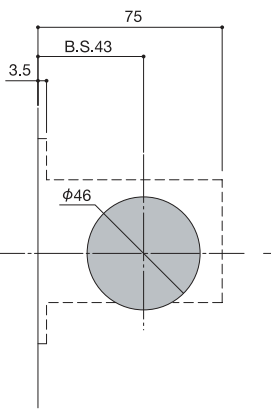
Cut out for 431 door pull
