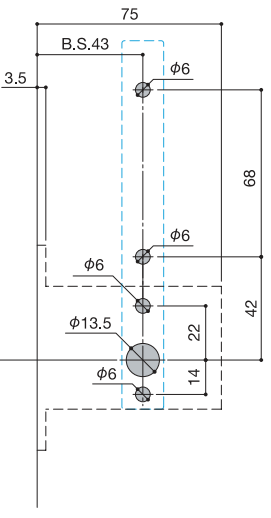
435 Cut out for lock case
