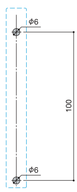
Cut out for 435 door pull
