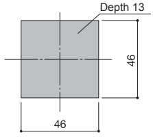
Cut out for 432 door pull
